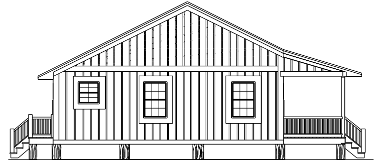
LEFT ELEVATION
