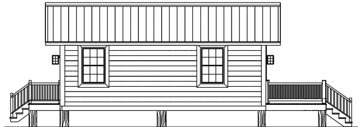
LEFT ELEVATION
